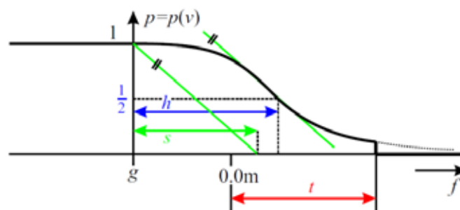
Figure 2: Mathematical principle of the filtering algorithm
